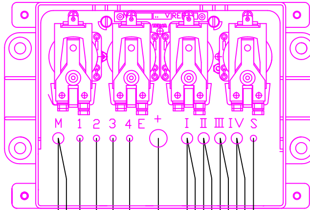
RELAY BOX JD331121 (12V)
